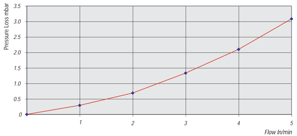
Pressure Loss 5 l/min (Air)
