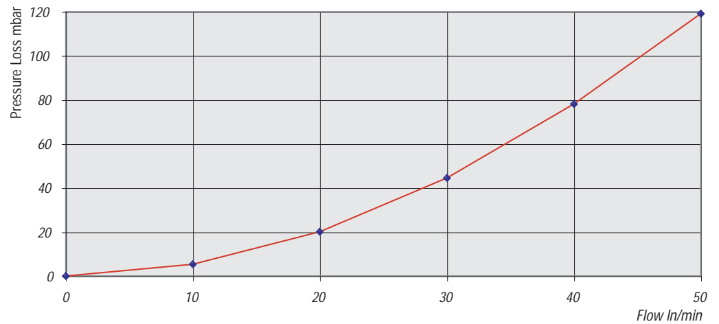
Pressure Loss 50 l/min (Air)
