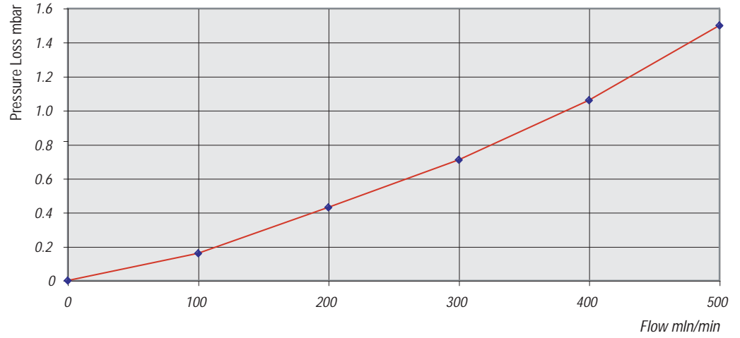
Pressure Loss 500 ml/min (Air)
